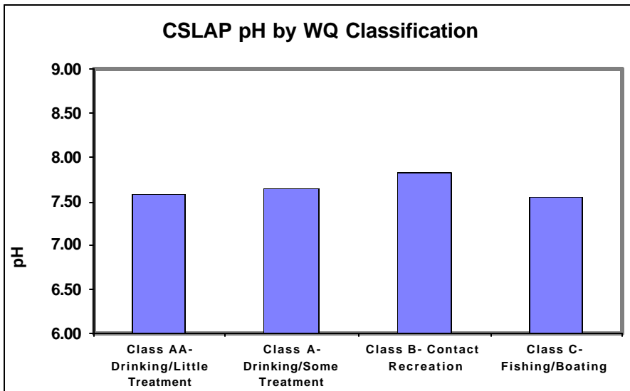
Figure 6d. pH in CSLAP Lakes by Lake Use
