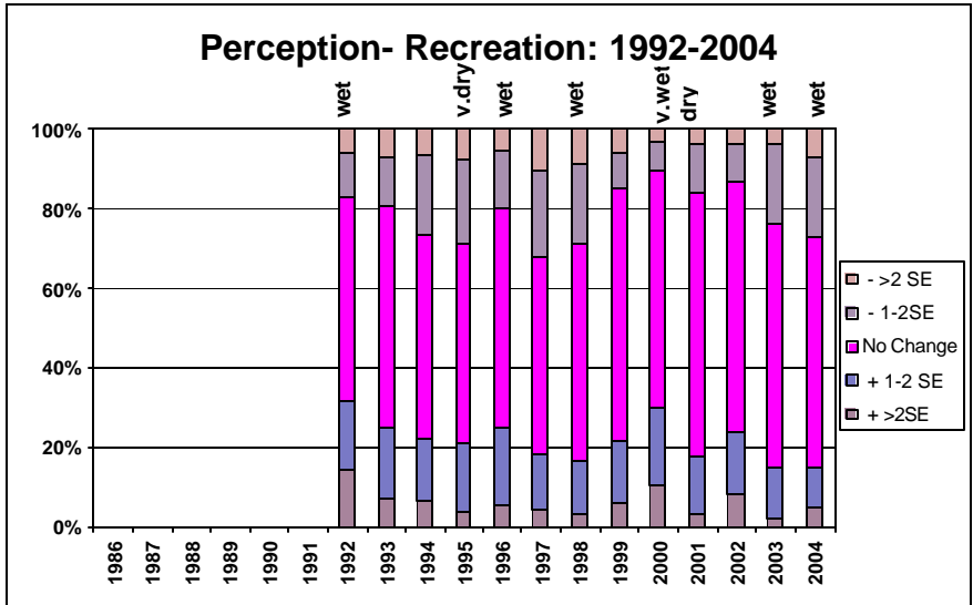
Figure 15a. Annual Change from “Normal” Recreational Assessment in CSLAP Lakes (SE = Standard Error)
