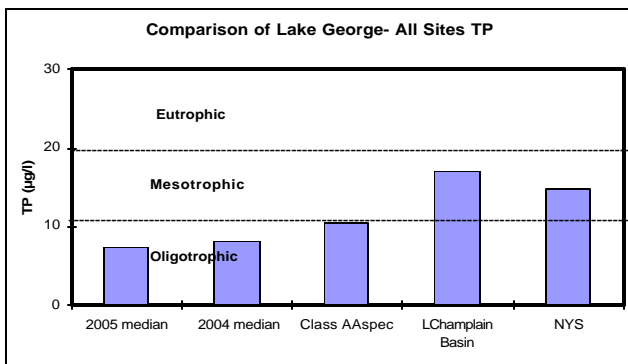
Figure 33. Comparison of 2005 Total Phosphorus to Lakes With the Same Water Quality Classification, Neighboring Lakes, and Other CSLAP Lakes in 2005
