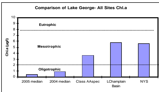
Figure 32. Comparison of 2005 Chlorophyll a to Lakes with the Same Water Quality Classification, Neighboring Lakes, and Other CSLAP Lakes in 2005
