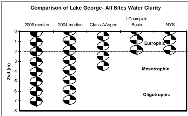
Figure 31. Comparison of 2005 Secchi Disk Transparency to Lakes With the Same Water Quality Classification, Neighboring Lakes, and Other CSLAP Lakes in 2005
