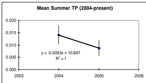
Figure 22a. Annual Average Summer Total Phosphorus for Lake George- S1
